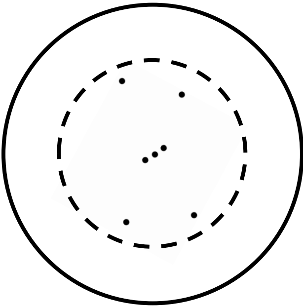
Orion (constellation)
