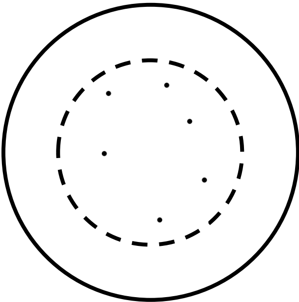
Auriga (constellation)
