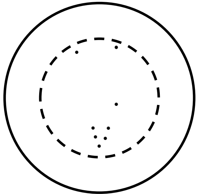
Taurus (constellation)
