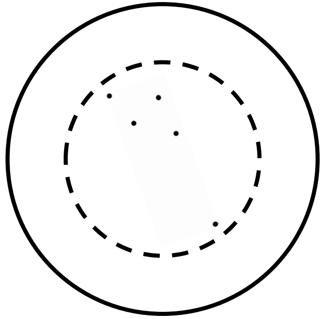
Delphinus (constellation)
