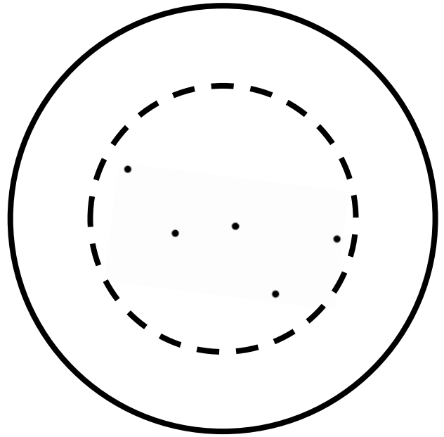
Cassiopeia (constellation)
