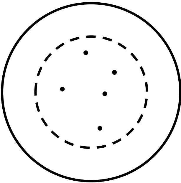
Crux (constellation)
